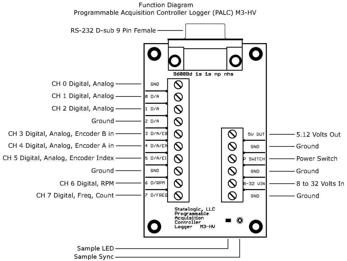
Figure 1: Connection Diagram
